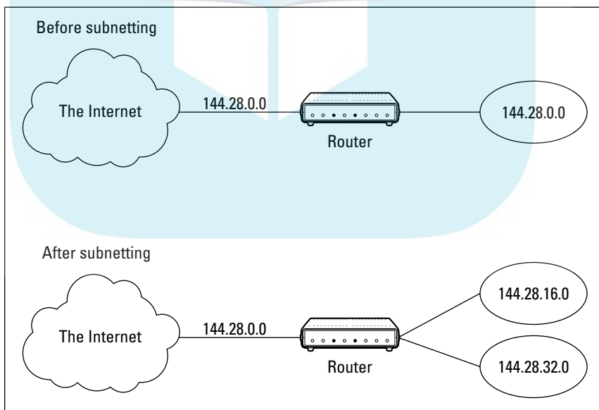
Figure 6-1: A network before and after sub- netting.
